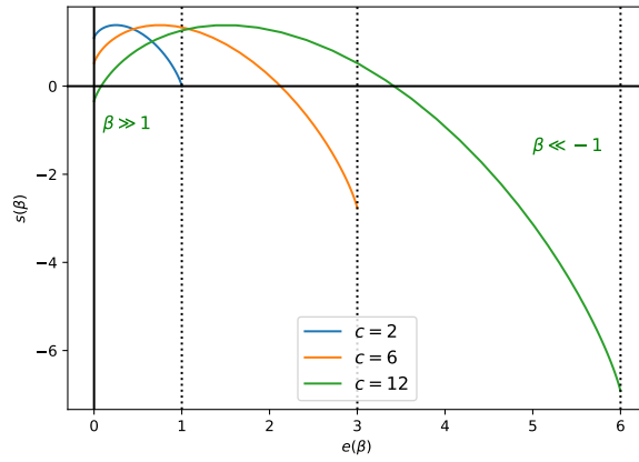
Figure 6.4.1: Entropy as a function on the energy cost for graph coloring with q = 4 colors corresponding to the paramagnetic fixed point of belief propagation. Average degree of the graph is c .
