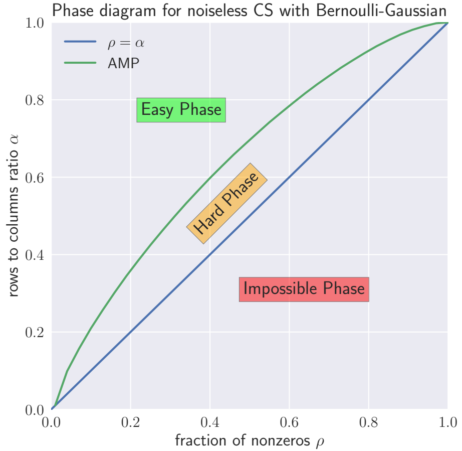
Figure 16.6.1: Phase diagram of noiseless compressed sensing for Gauss-Bernulli prior
